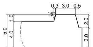
Detail D
