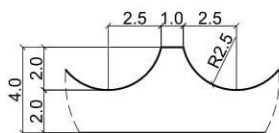
Detail B
